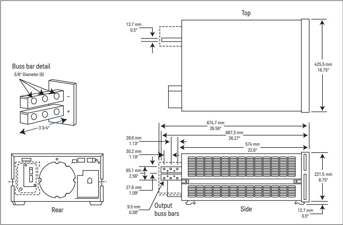
Keysight models: 6690A, 6691A, 6692A
